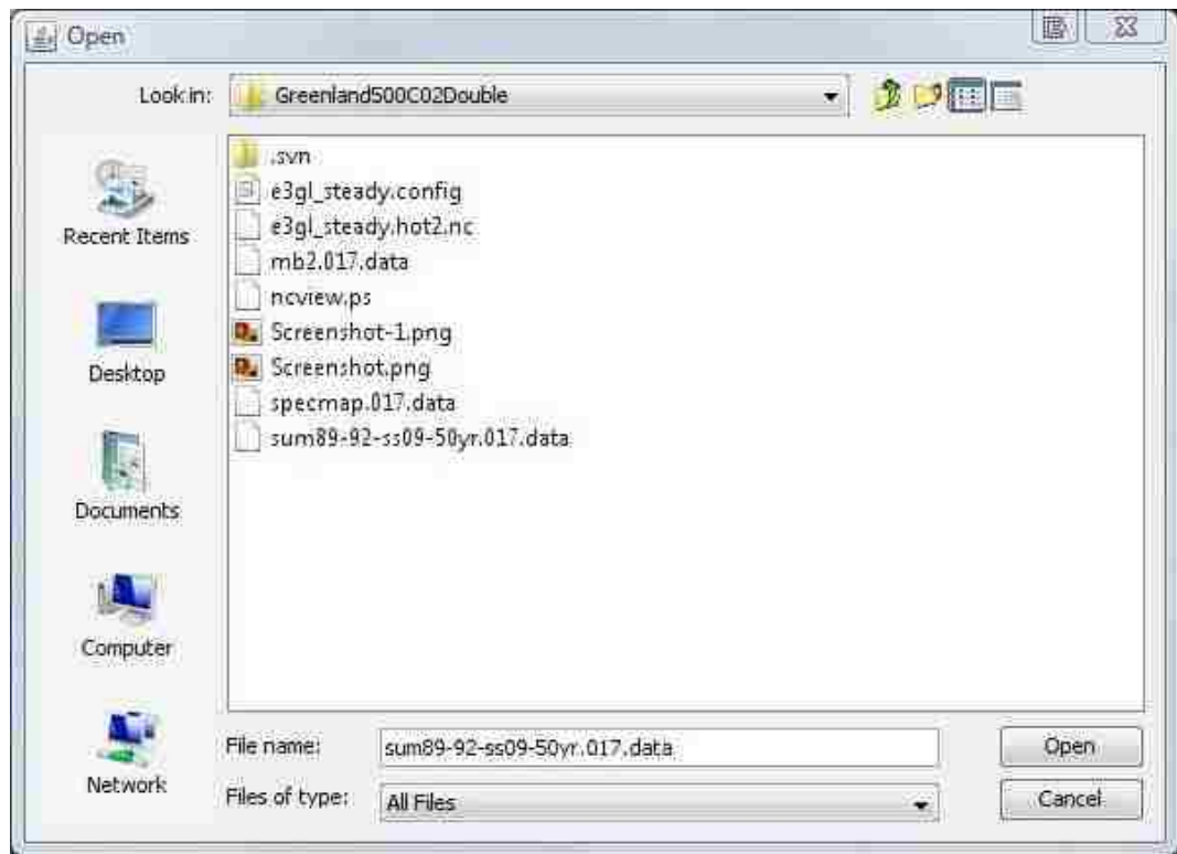
Figure 9 File Dialog
